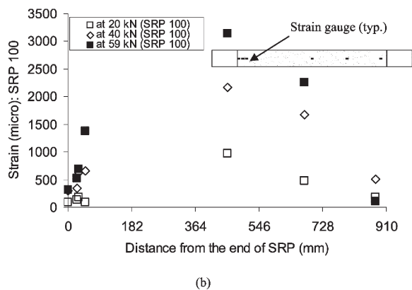
Figure 5 – SRP strains at various load levels: (a) load vs. mid-span SRP strains; (b) typical strain distribution along the SRP sheet (SRP 100)
